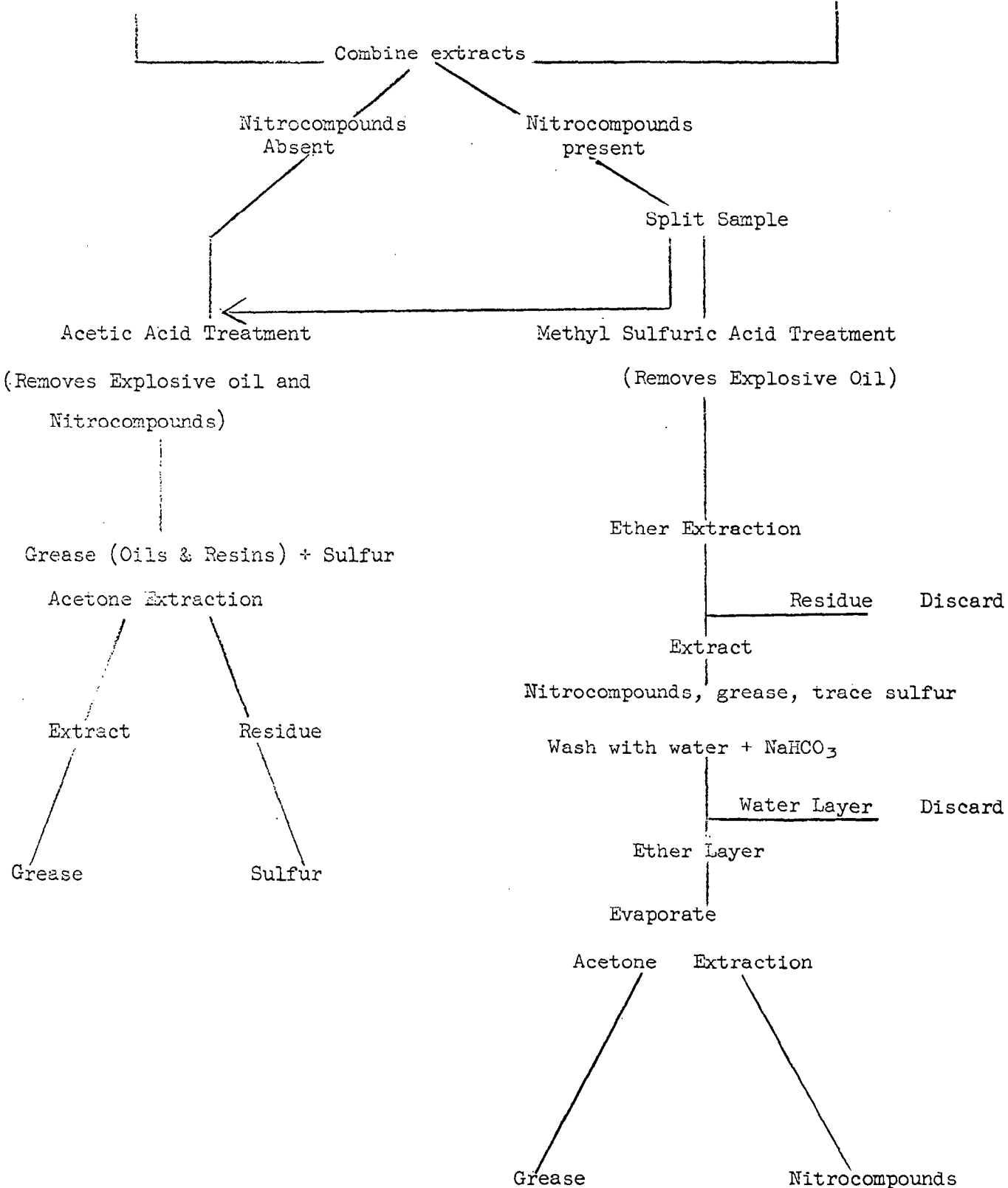
Figure 2 Determination of Ether Solubles
